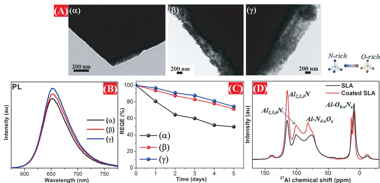
Figure 2. A) TEM images, B) PL spectra, and C) REQE of SLA with various TEOS contents: 0.0 (α), 3.0 (β), and 6.0 mM (γ). The internal and external QE were measured after aging under HT and HH conditions by excitation with 460 nm light. D) 27 Al solid-state NMR spectra showing the oxygen content in the crystal structure of SLA (black line) and coated SLA (red line).
